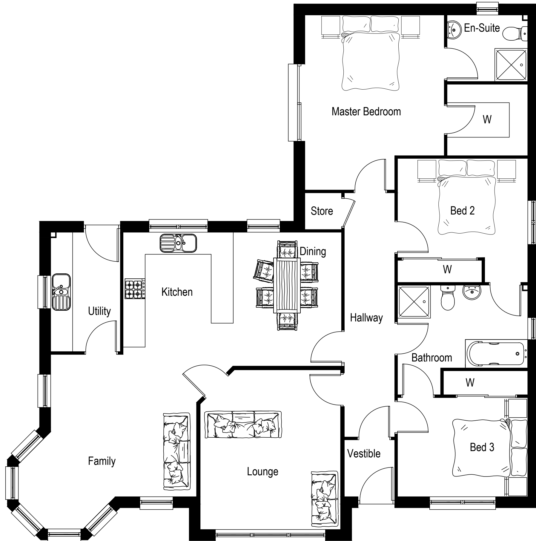
Ground Floor Plan Ground Floor Area (135.7sqm)
